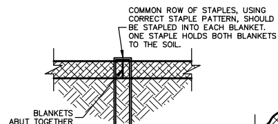
SIDE SEAM ABUT STAPLE DETAIL NO SCALE
