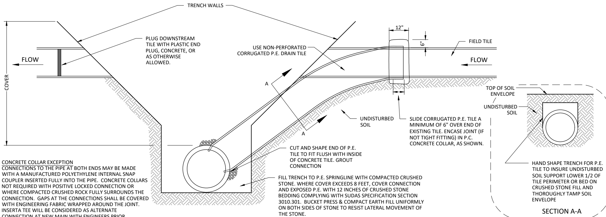
TYPICAL FIELD TILE CONNECTION
